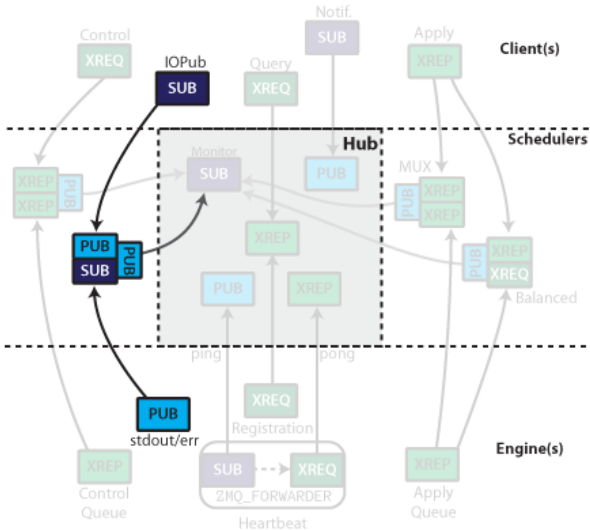
Figure 7.5: stdout/err are published via a PUB/SUB MonitoredQueue
